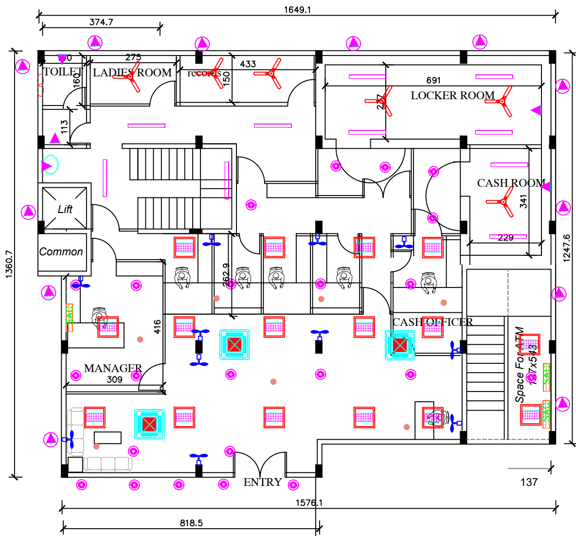
PROPOSED LAYOUT OF CHERANALLUR BRANCH - GROUND FLOOR
